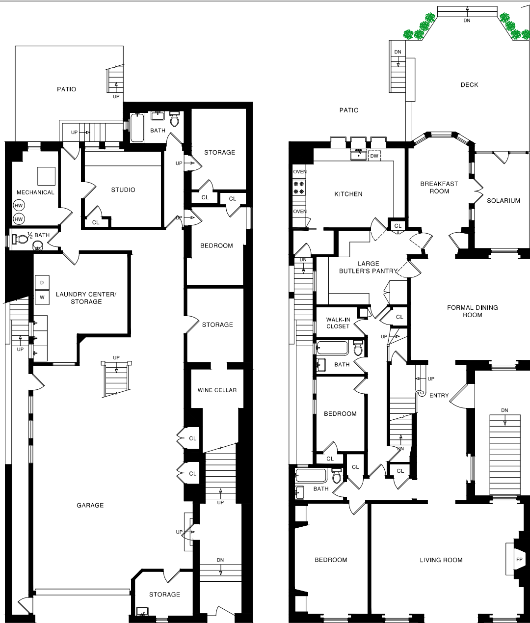
LOWER LEVEL
